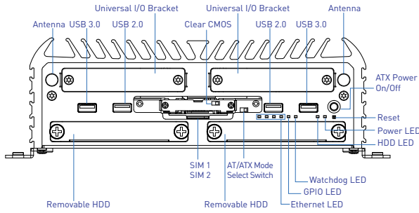
Front Panel
