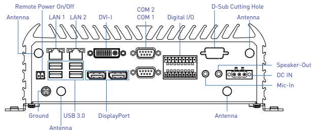
Rear Panel
