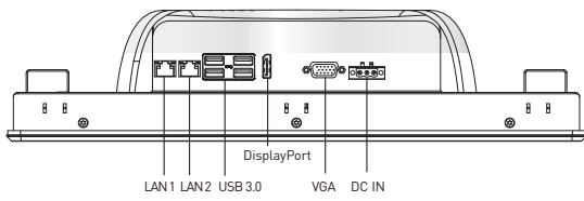
Rear I/O
